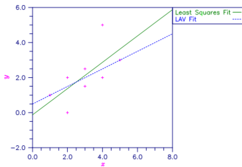
Figure 11, Least Squares and Least Absolute Value Fitted Lines
