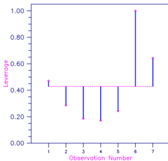
Figure 6, Plot of Leverages h_i and the Average ( p/n = 3/7 )
