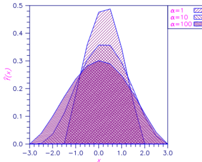
Figure 20, Density Estimates Using \alpha = 1, 10, 100
